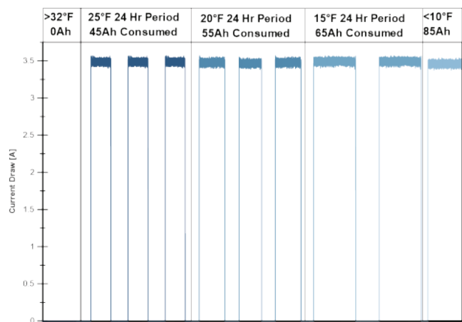
BBGC3iH Integrated Heater Draw Expected in a 24Hr Period
