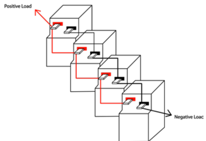
Four batteries connected in parallel to create a 12V 400Ah battery bank
