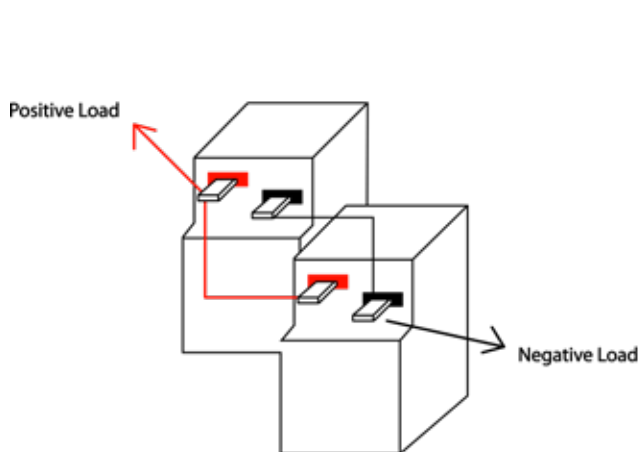
Two batteries connected in parallel to create a 12V 200Ah battery bank
