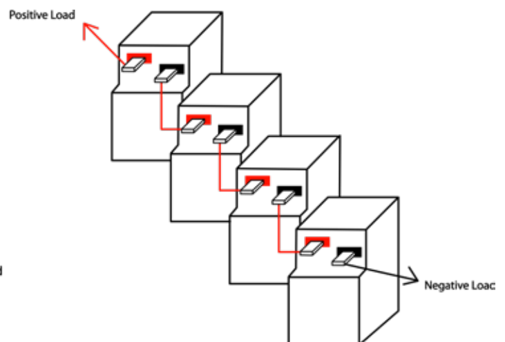
Four batteries connected in series to create a 48V 100Ah battery bank
