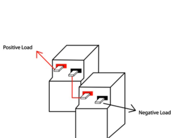
Two batteries connected in series to create a 24V 100Ah battery bank
