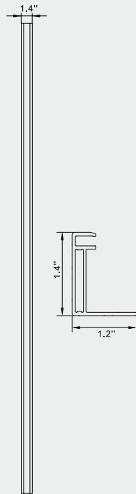
Side Profile
