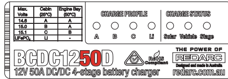
Figure 1.1.1 - The BCDC1250D Front Panel
