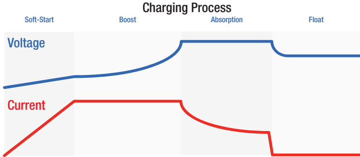
Figure 1.3.4.1 - Charging Process
