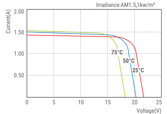
DFE200S-24U I-V Curves
