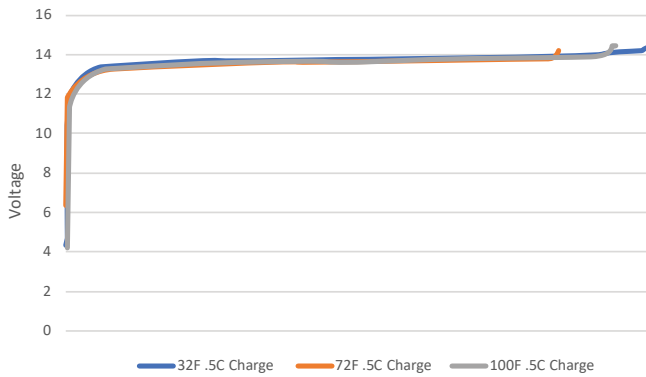
.5C State of Charge with Temperature Variations
