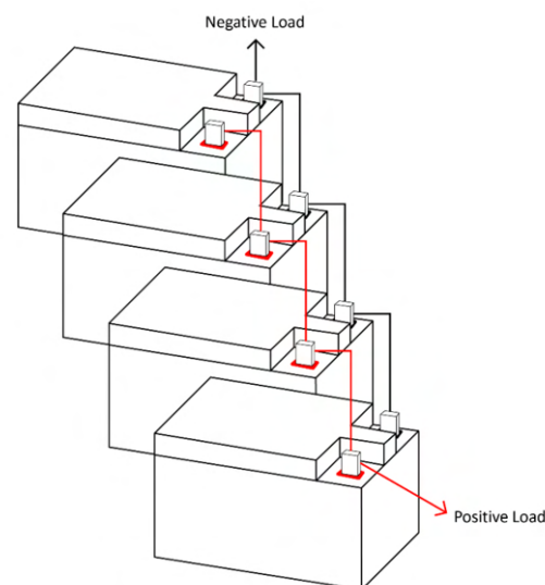
Four batteries connected in parallel to create a 24V 200Ah battery bank
