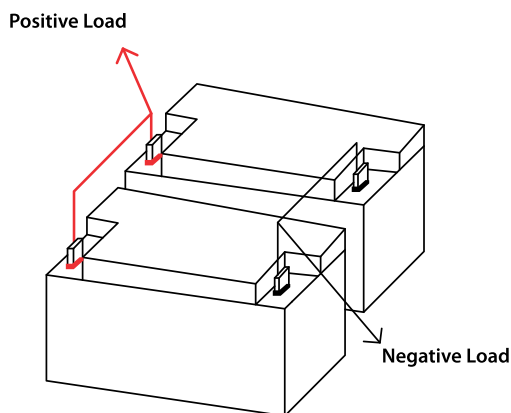
Two batteries connected in parallel to create a 12V 200Ah battery bank
