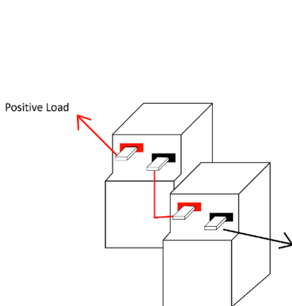
Figure 4.1: Two GC2|GC2H Batteries connected in Series to create a 24V 100Ah Batter Bank
