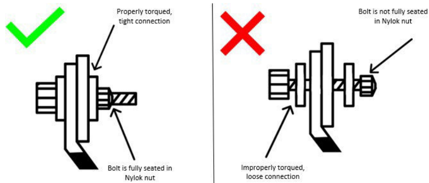
Figure 2: Proper and Improper Terminal Connections
