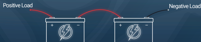
Series Connection 24V 100Ah Bank Increases Voltage, Ah stays the same.
