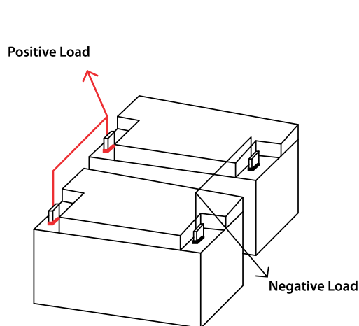
Two batteries connected in parallel to create a 12V 150Ah battery bank
