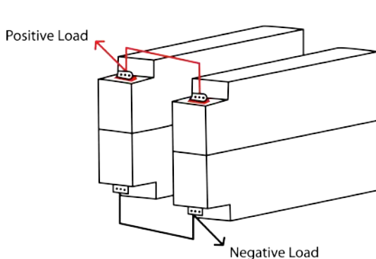
Two GC3 Batteries connected in Parallel to create a 12V 540Ah Battery Bank
