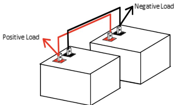
Figure 3: Two 8D Batteries connected in Parallel to create a 12V 540Ah Battery Bank
