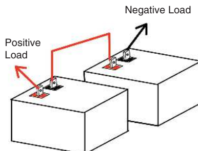
Series Connection, 24V 270Ah bank Increases Voltage, Ah stays the same.
