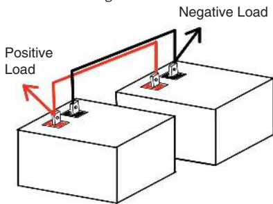
Parallel Connection, 12V 540Ah bank Increases Ah, Voltage stays the same.
