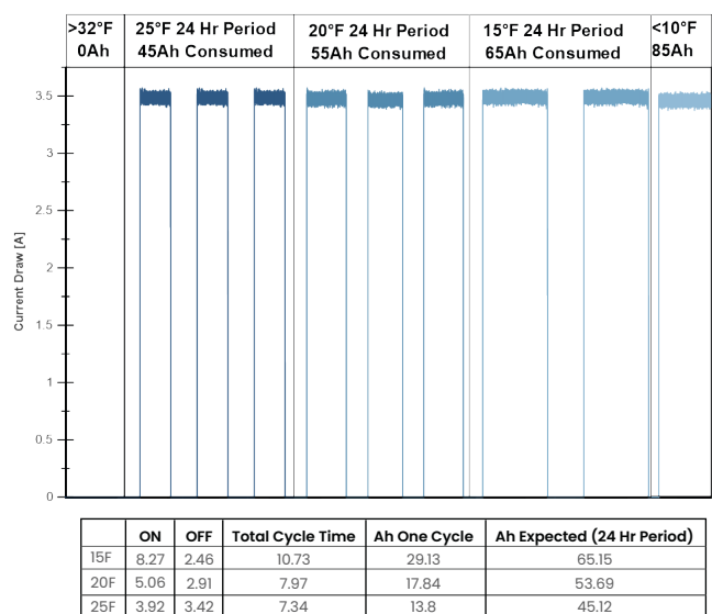
BBGC3iH Integrated Heater Draw Expected in a 24Hr Period
