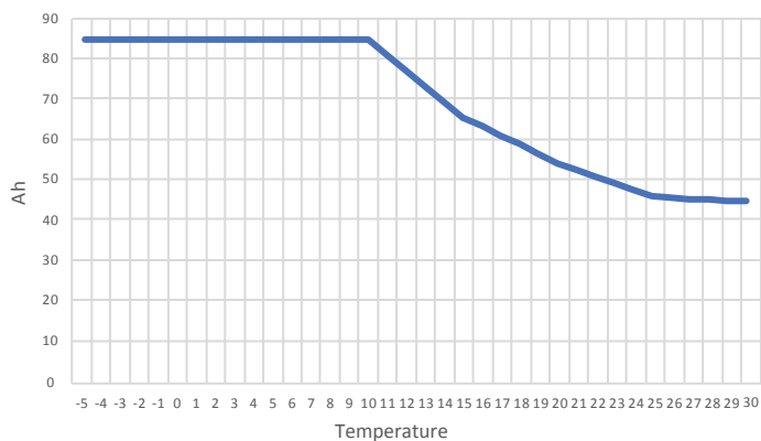
BBGC3iH Integrated Heater Draw Expected in a 24Hr Period
