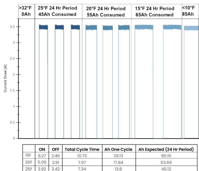
BBGC3H Integrated Heater Draw Expected in a 24Hr Period
