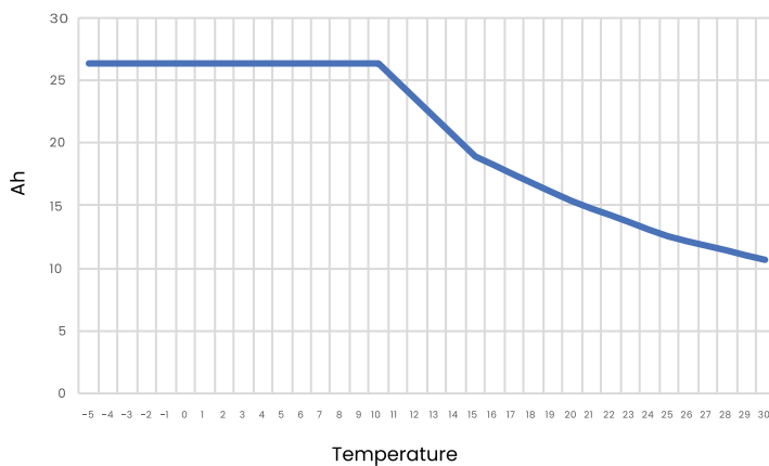
BB5024H Integrated Heating Draw Expected in a 24Hr Period
