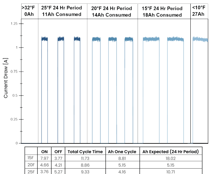
BB5024H Integrated Heating Draw Expected in a 24Hr Period
